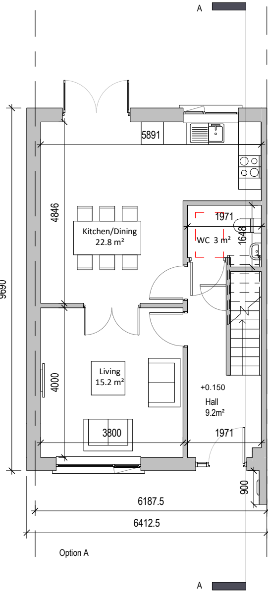
1 Ground Floor Mid Terrace & End of Terrace (Layout Options A,B&C) 1 : 100
