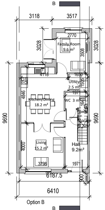
3 Ground Floor Options A & B with Extension 1 : 200
